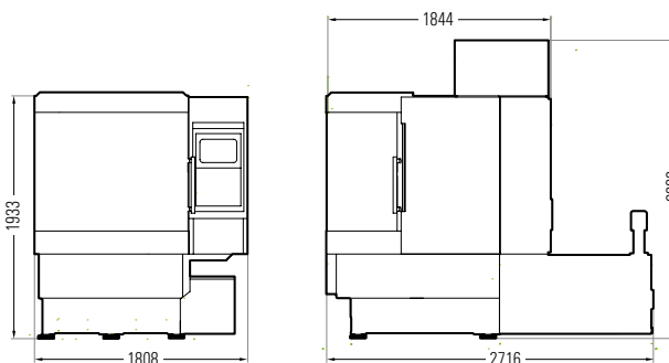
HELITRONIC ESSENTIAL (Dimensions en mm)
